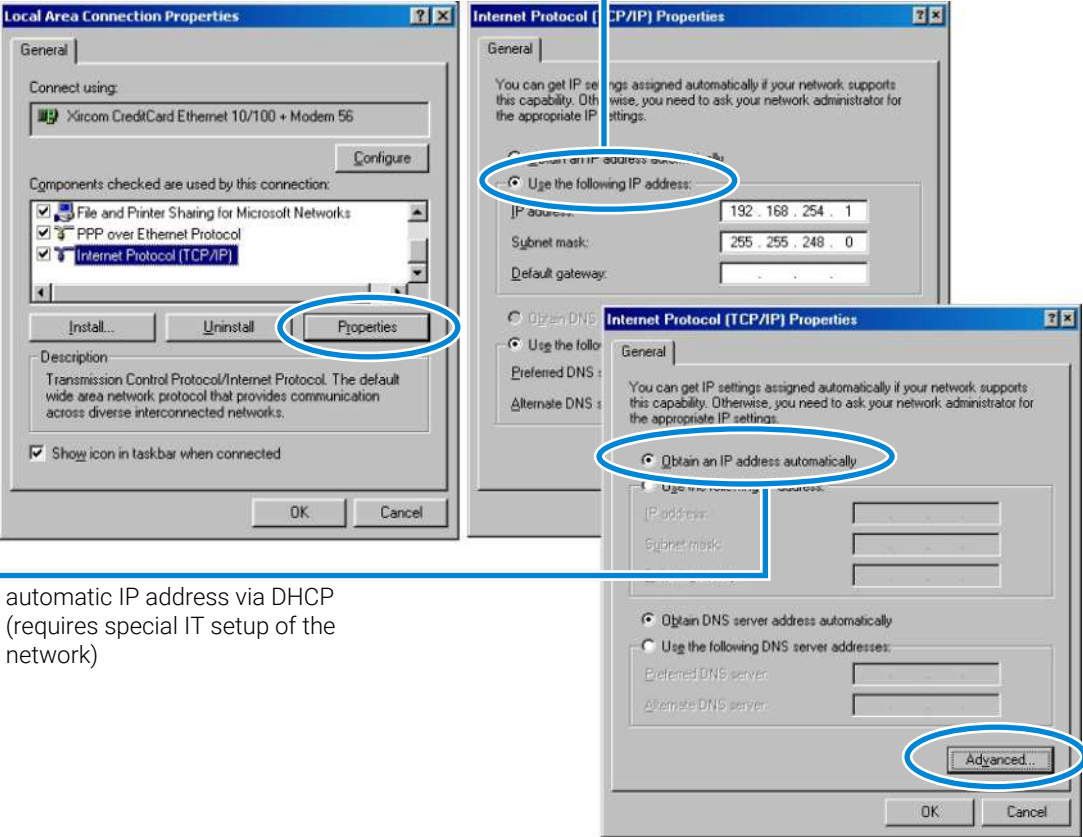
Figure 45: Changing the TCP/IP settings of the PC
