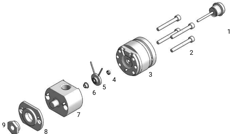
G7131-60640 (Secondary Pump Head Assembly biocompatible)
