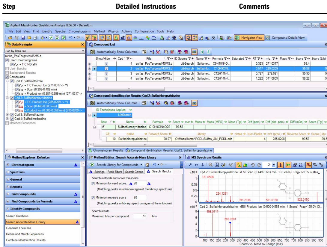
Figure 63 Results after running the Search Accurate Mass Library algorithm.
