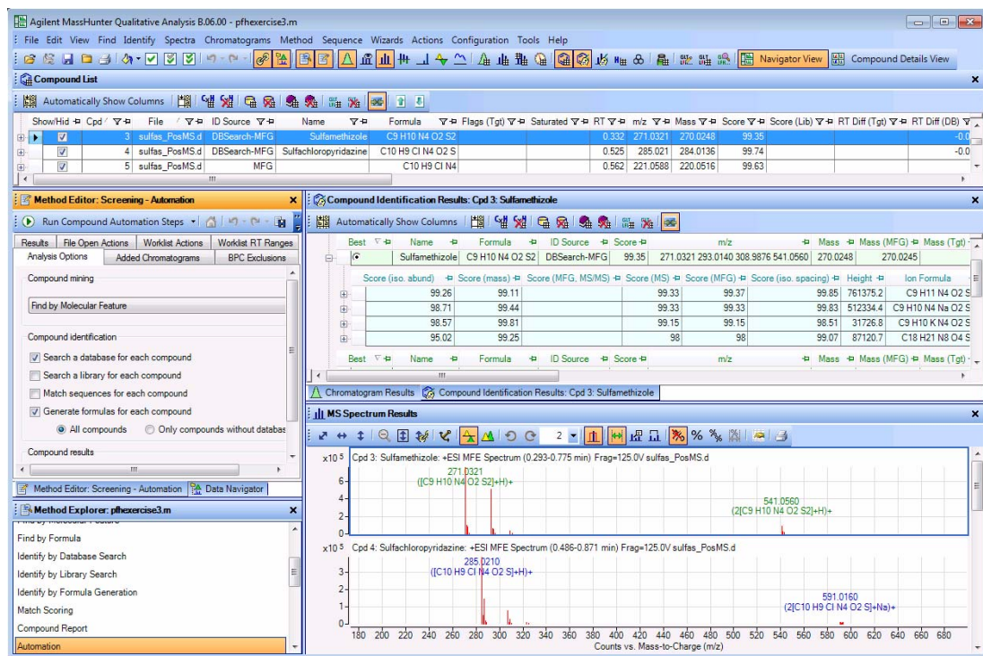
Figure 71 Tabbed results from running compound automation identification steps
