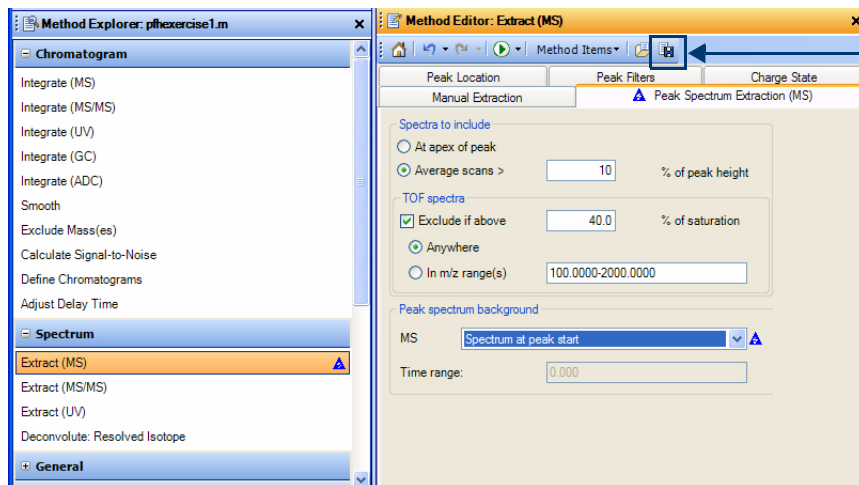
Figure 66 The Spectrum > Extract (MS) > Peak Spectrum Extraction (MS) tab
