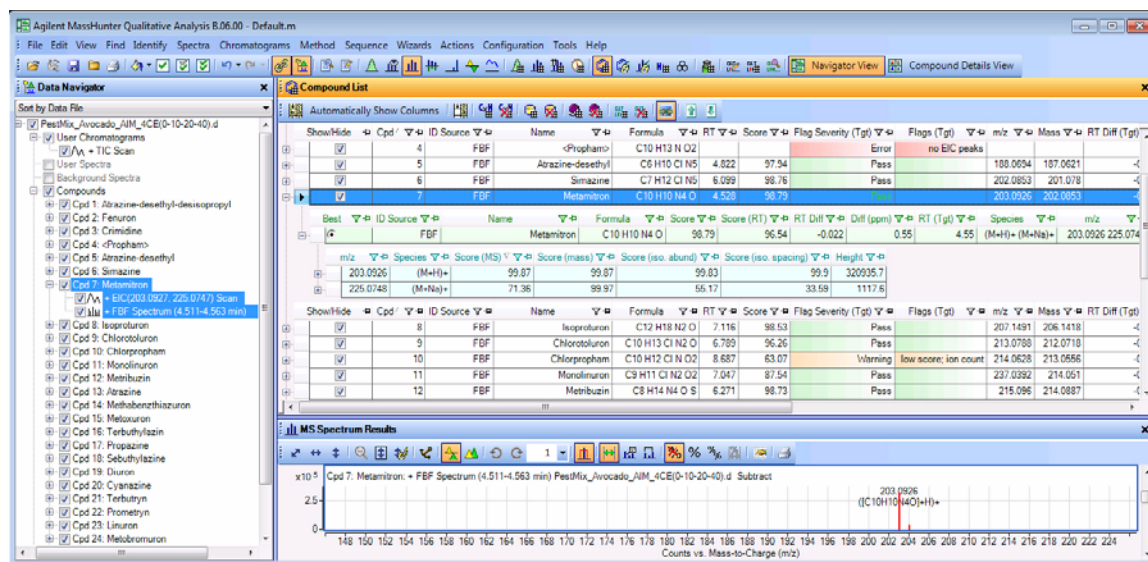
Figure 87 Find by Formula results in the Data Navigator, Compound List, and MS Spectrum Results windows.
