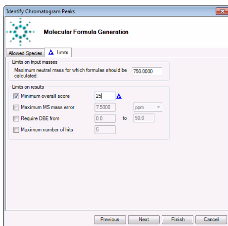
Figure 80 The Molecular Formula Generation page in the Identify Chromatogram Peaks wizard
