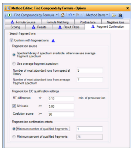
Figure 89 The Find Compounds by Formula > Fragment Confirmation tab
