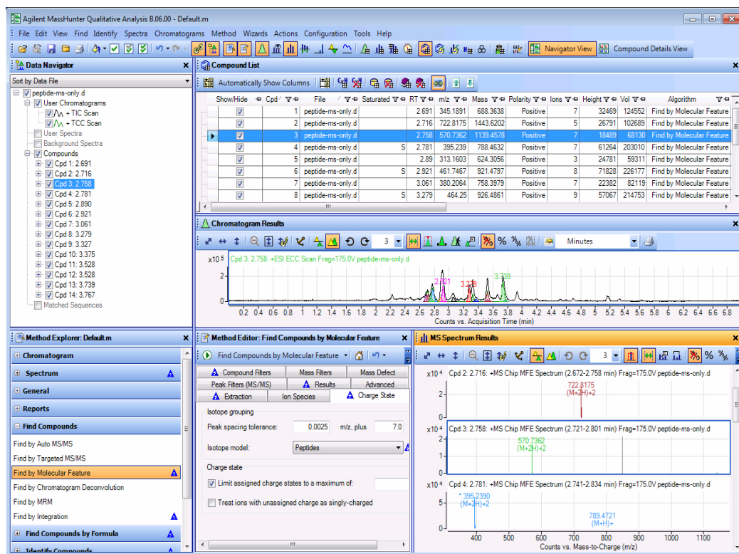
Figure 54 Find Compounds by Molecular Feature with Qualitative Analysis
