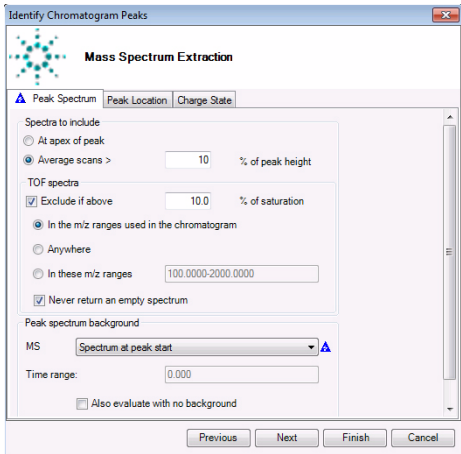
Figure 77 The Mass Spectrum Extraction page in the Identify Chromatogram Peaks wizard
