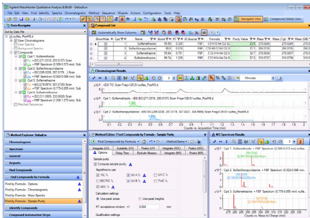
Figure 53 Finding all four compounds in the sulfa drug mix
