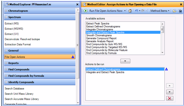
Figure 67 The General > File Open Actions section in the Method Editor
