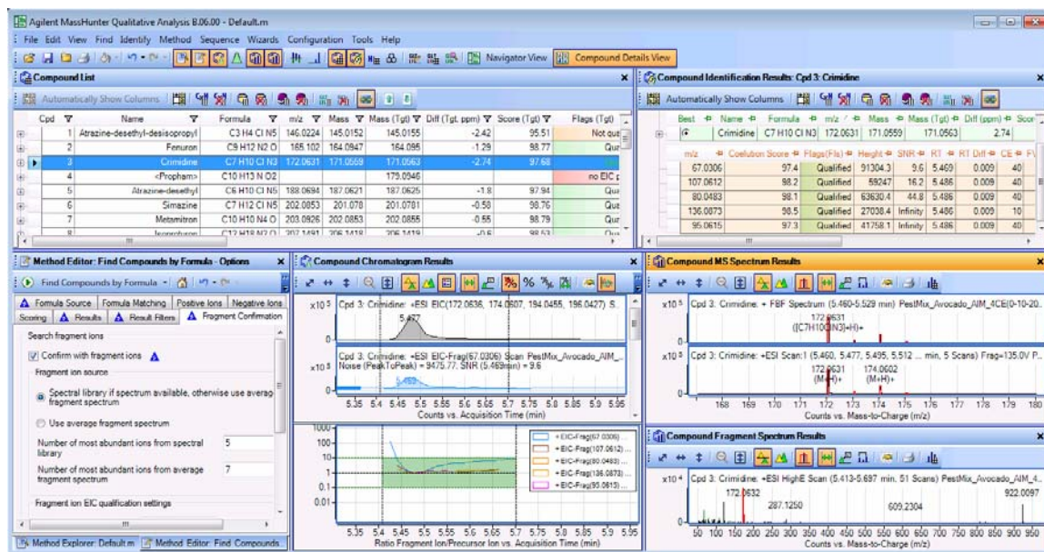
Figure 93 Compound List window with three new columns for fragment ions
