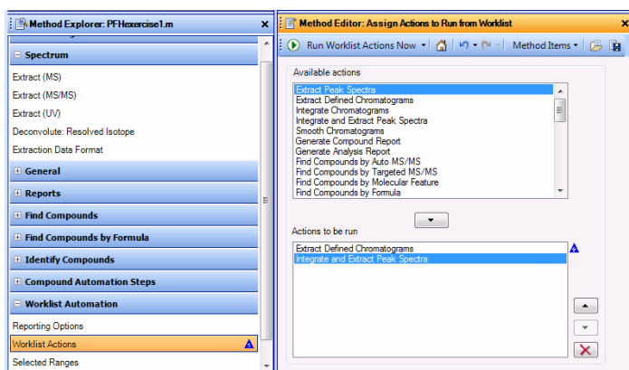
Figure 68 The Worklist Automation > Worklist Actions section in the Method Editor
