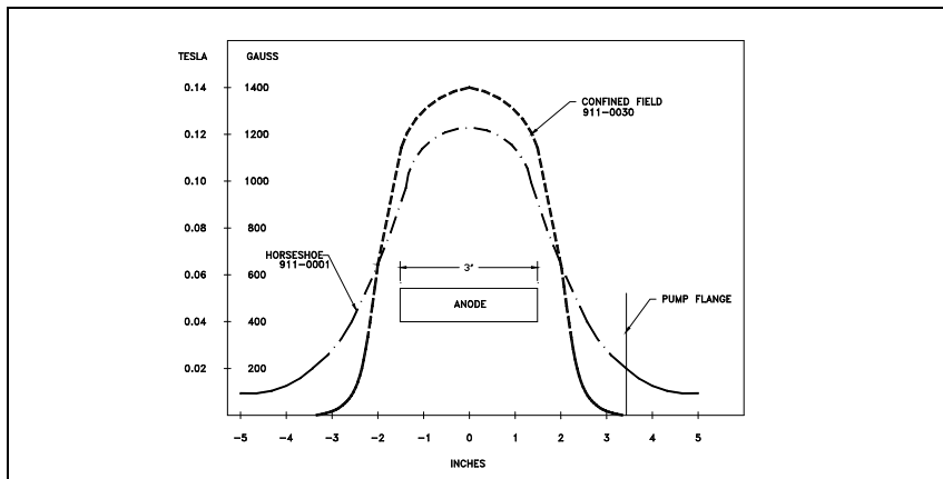
Figure 6 Magnetic field in gap of horseshoe and confined field magnets
