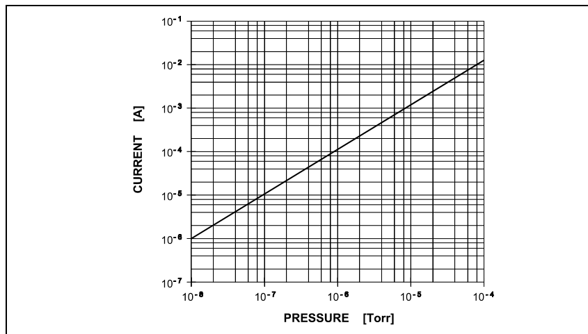
Figure 4 Pressure vs current diagram
