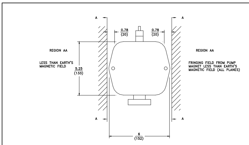
Figure 7 8 l/s pump magnet field free region
