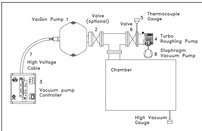
Figure 10 Typical installation
