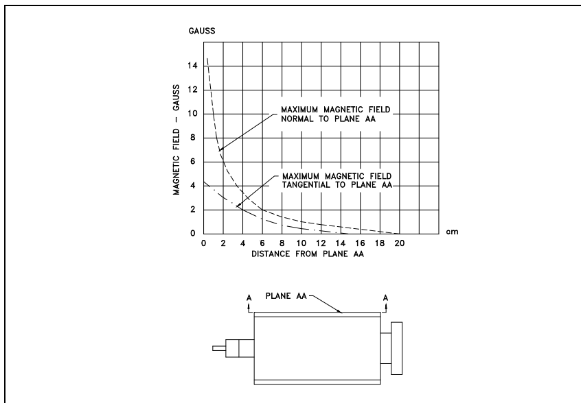
Figure 9 Magnetic field at flat of pump magnet package
