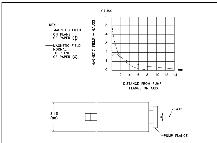
Figure 8 Magnetic field on pump flange axis
