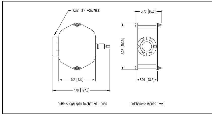
Figure 5 8 l/s VacIon pump outline drawing
