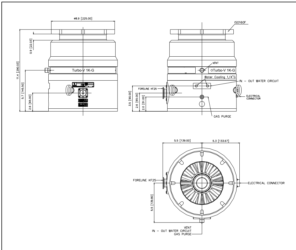
Figure 3 869-8961 (ISO 160 F inlet flange – KF25 foreline flange)
