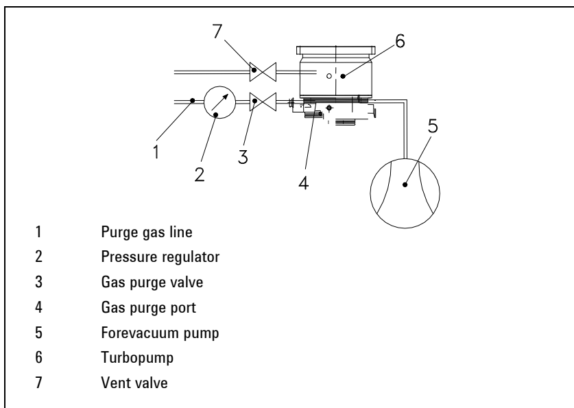
Figure 39 Purge layout
