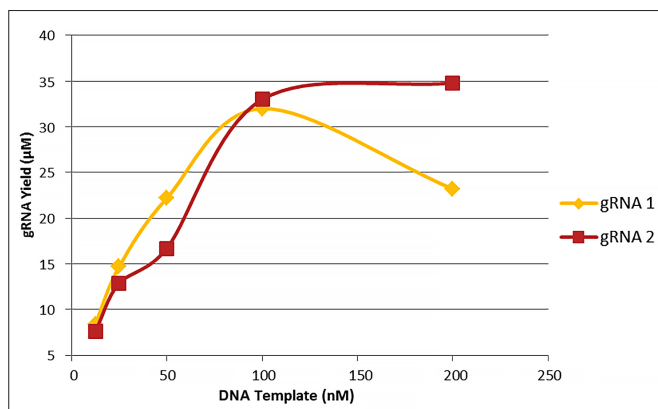
Figure 1. The effect of template input on yield of gRNA. Decreasing concentrations of template were subjected to 1 hour of in vitro transcription, showing that even low concentrations of template DNA are sufficient to obtain high yields of gRNA.
