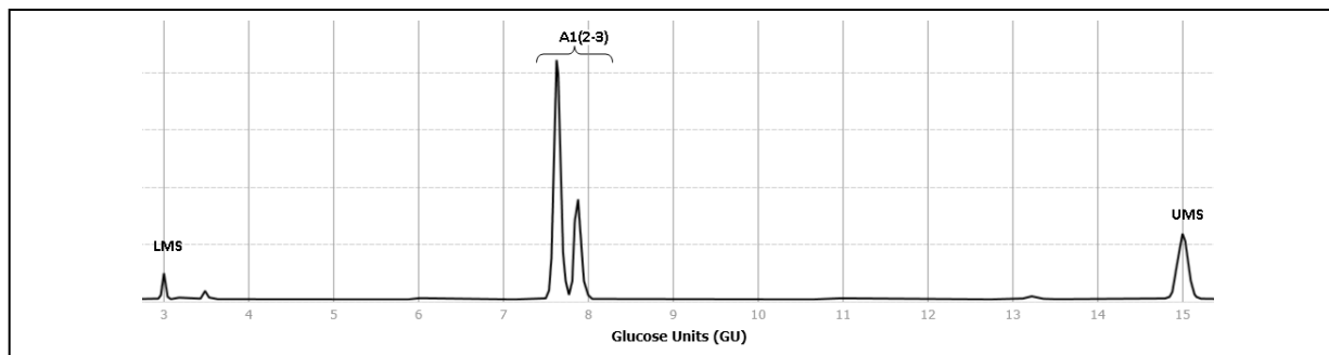
Figure 1 – Gly-Q Results: The InstantQ-labeled standard is injected onto a Gly-Q CE Instrument (GQ2100) under the conditions and method below (see Directions for Use for recommended amounts). Gly-Q Migration Standards (GKSQ-500) are co-injected with the glycan:
