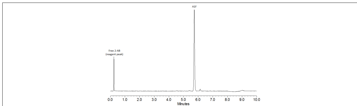
Figure 1 - UPLC® Results: 3 - 6 pmol (1 \mu l) of the 2-AB-labeled 4 glycan was injected on a Waters ACQUITY UPLC® H Class System utilizing a 10-minute method under the conditions below:
