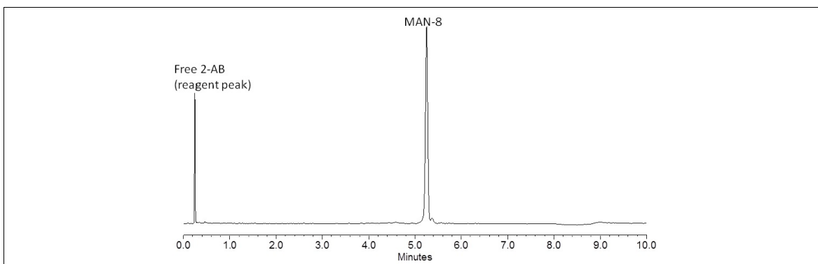
Figure 1 - UPLC® Results: 3 - 6 pmol (1 \mu l, aqueous) of the 2-AB-labeled 4 glycan was injected on a Waters ACQUITY UPLC® H Class System utilizing a 10-minute method under the conditions below:
