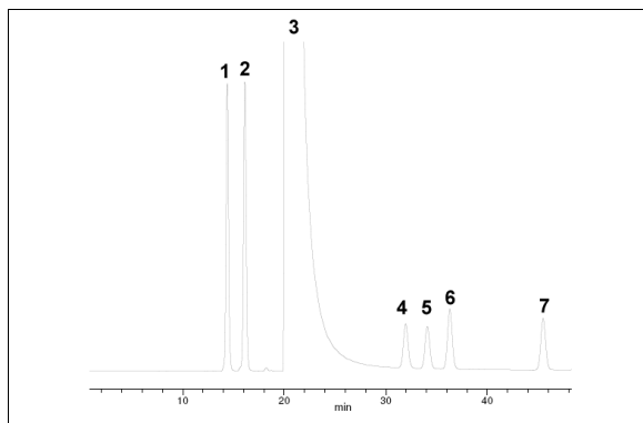
Figure 1 - HPLC of 2-AA labeled Monosaccharide Standard Set
