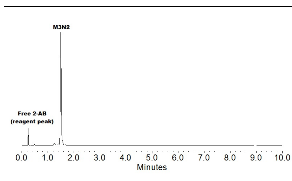
Figure 3 - M3N2 labeled with 2-AB and analyzed on a Waters ACQUITY® UPLC® BEH Glycan column (1.7 μm, 2.1 x 100 mm) in ammonium formate/acetonitrile.
