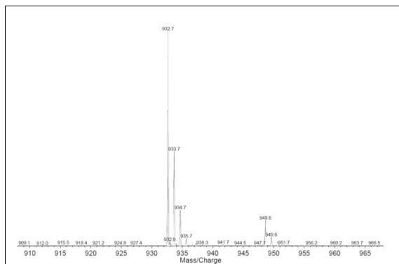
Figure 2 - MALDI-TOF MS of M3N2 [M+Na] +
