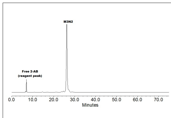
Figure 1 - HPLC results: M3N2 labeled according to the Signal™ 2-AB Labeling Kit (GKK-404) and analyzed on a GlycoSep™ N column (GKI-4728) in ammonium formate/acetonitrile.
