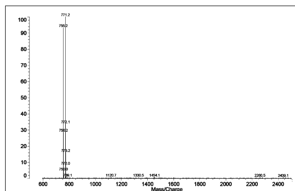
Figure 2 - MALDI-TOF MS of MNNF [M+Na] +
