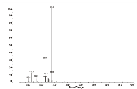
Figure 2 - MALDI-TOF of NF [M + Na] +
