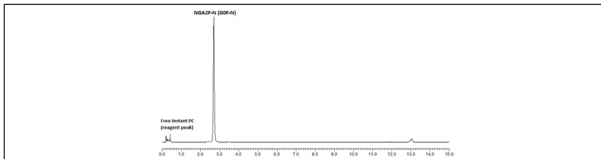
Figure 1 - UPLC® Results: 1 µl, aqueous of the InstantPC-labeled glycan was injected on a Waters ACQUITY UPLC® H Class System utilizing a 15-minute method under the conditions below:
