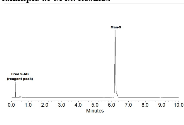
Figure 3 - Man-9 labeled with 2-AB and analyzed on a Waters ACQUITY® UPLC® BEH Glycan column (1.7 μm, 2.1 x 100 mm) in ammonium formate/acetonitrile.
