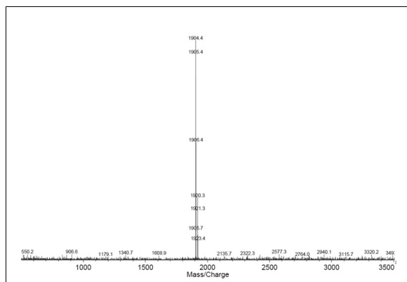
Figure 2 - MALDI-TOF MS of Man-9 [M+ Na] +
