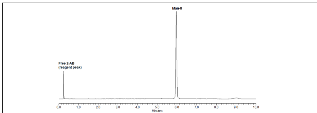
Figure 1 - UPLC® Results: 3 - 6 pmol (1 µl, aqueous) of the 2-AB-labeled 4 glycan was injected on a Waters ACQUITY UPLC® H Class System utilizing a 10-minute method under the conditions below:
