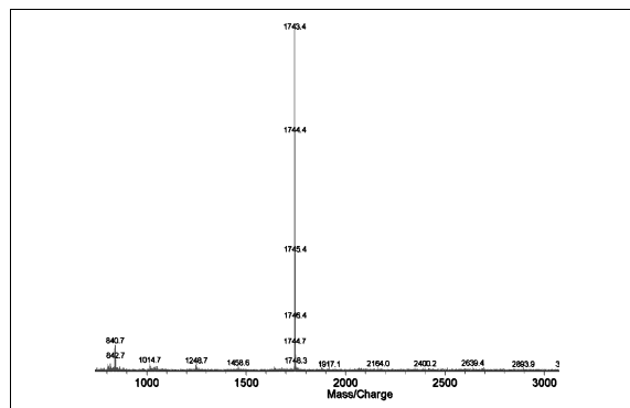
Figure 2 - MALDI-TOF of Man-8 [M + Na] +
