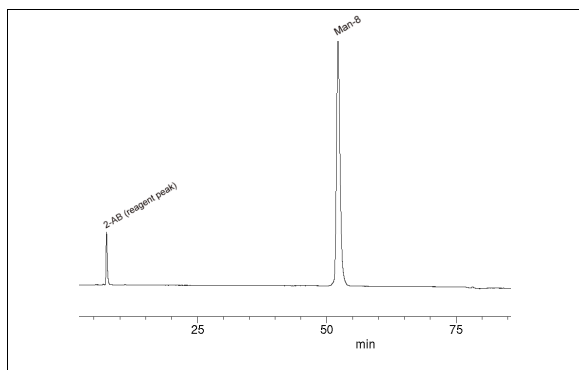
Figure 1 - HPLC of 2-AB labeled Man-8
