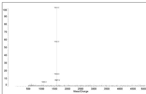
Figure 2 - MALDI-TOF of Man-7 [M + Na] +
