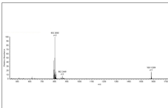
Figure 2 - ESI-MS of Man-7
