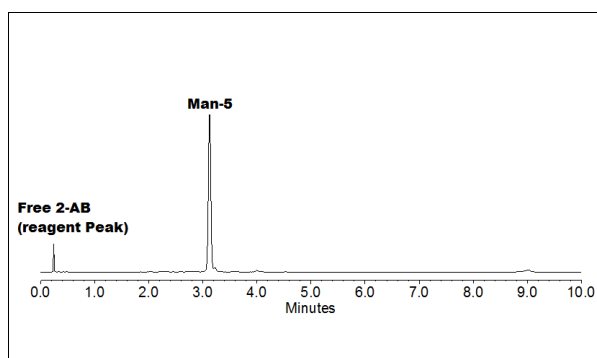
Figure 3 - MAN-5 labeled with 2-AB and analyzed on a Waters ACQUITY® UPLC® BEH Glycan column (1.7 μm, 2.1 x 100 mm) in ammonium formate/acetonitrile.
