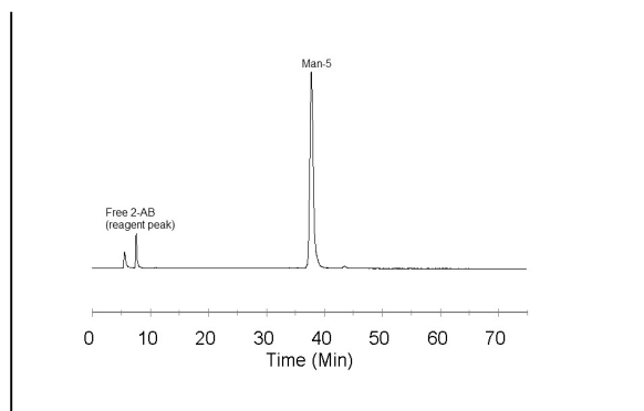
Figure 1 - HPLC results:
