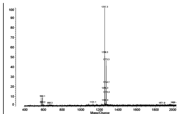
Figure 2 - MALDI-TOF MS of Man-5 [M+Na] +
