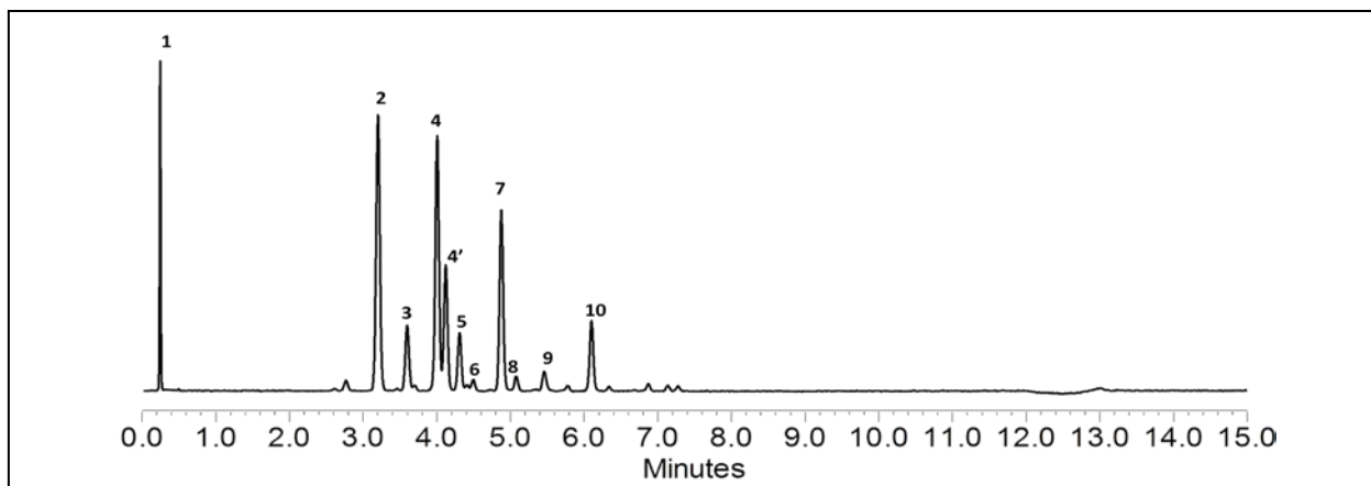
Figure 1 - UPLC® Results: 9.4 pmol (1 µl, aqueous) of the 2-AB-labeled library was injected on a Waters ACQUITY UPLC® H Class System utilizing a 15-minute method under the conditions below:
