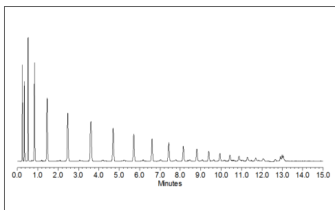
Test-labeled Oligosaccharide
