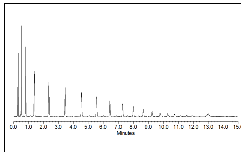
Reference Labeled Oligosaccharide
