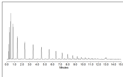
Reference Labeled Oligosaccharide
