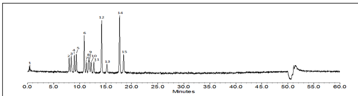
Figure 1 - UPLC® Results: 3 -6 pmol (1 µl, aqueous) of the InstantAB-labeled glycan library was injected on a Waters ACQUITY UPLC® H Class System utilizing a 60-minute method under the conditions below (see Table 1 for peak ID; the number of peaks observed depends on the running conditions employed):
