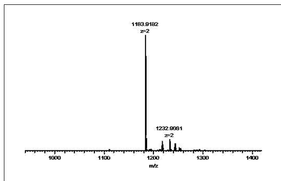
Figure 2 - ESI-MS of A2F [M - 2H]^{2-}
