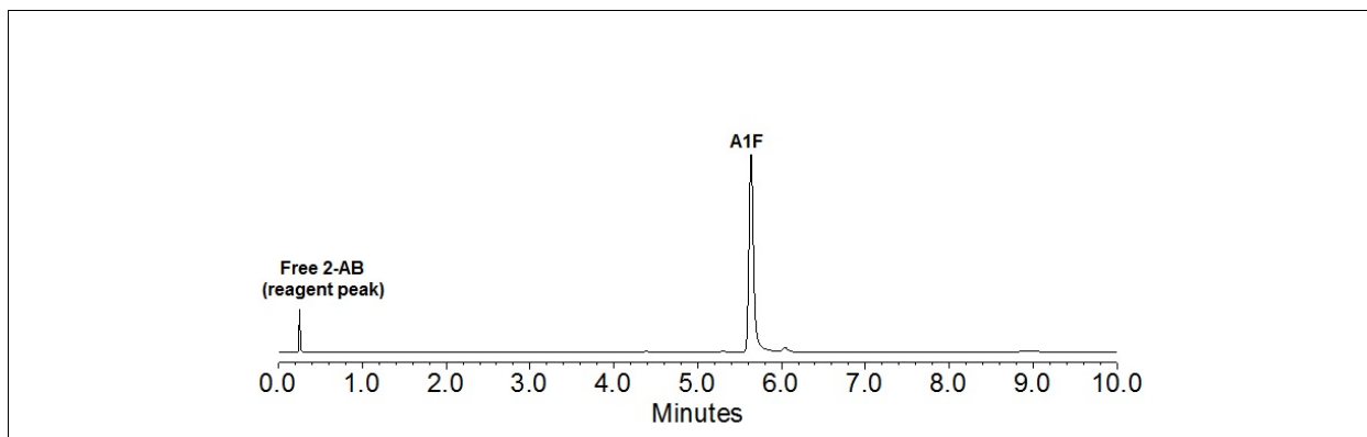
Figure 1 - UPLC® Results: 3 - 6 pmol (1 \mu l, aqueous) of the 2-AB-labeled glycan was injected on a Waters ACQUITY UPLC® H Class System utilizing a 10-minute method under the conditions below:
