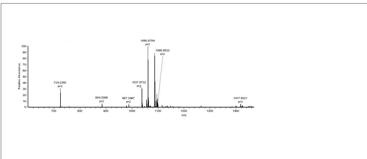
Figure 2 - Mass Spectrum of A1F
