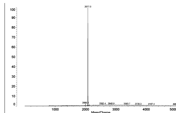
Figure 2 - ESI-MS of A1F [M - 2H] 2-
