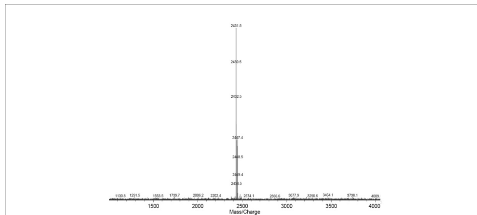
Figure 2 - Mass Spectrum of A1
