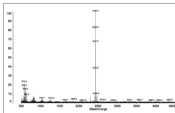
Figure 2 - MALDI-TOF MS of permethylated A1 [M+Na] +
