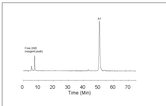
Figure 1 - HPLC results: A1 labeled according to the Signal™ 2-AB Labeling Kit (GKK-404) and analyzed on a GlycoSep™ N column (GKI-4728) in ammonium formate/acetonitrile.
