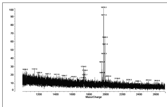
Figure 2 - MALDI-TOF MS of A1 [M-H+2Na] +
