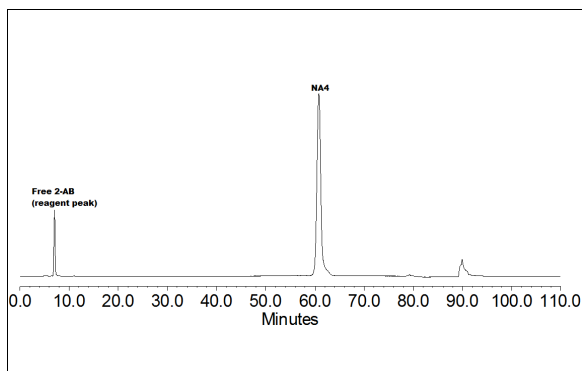
Figure 1 - HPLC results: NA4 labeled according to the Signal™ 2-AB Labeling Kit (GKK-404) and analyzed on a GlycoSep™ N column (GKI-4728) in ammonium formate/acetonitrile.
