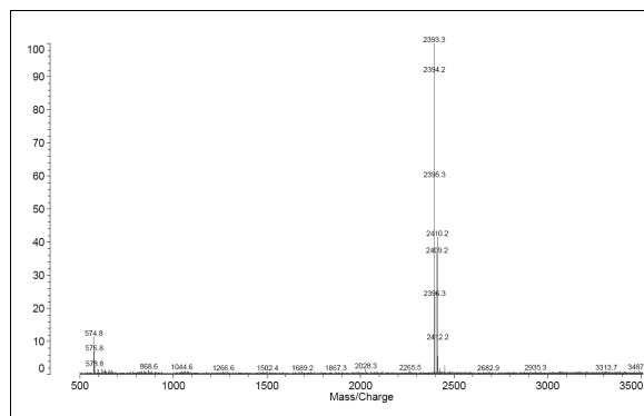
Figure 2 - MALDI-TOF MS of NA4 [M+Na] +
