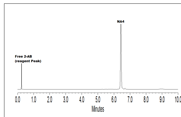
Figure 3 - Example of UPLC results: NA4 labeled with 2-AB and analyzed on a Waters ACQUITY® UPLC® BEH Glycan column (1.7 μm, 2.1 x 100 mm) in ammonium formate/acetonitrile.
