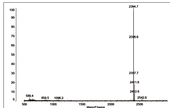
Figure 2 - MALDI-TOF of NA4 [M + Na] +
