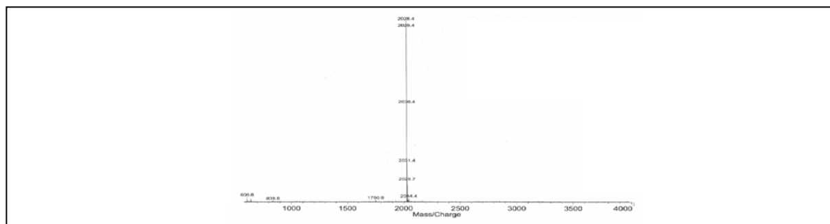
Figure 2 - Mass Spectrum of NA3 [ M + Na ] +
