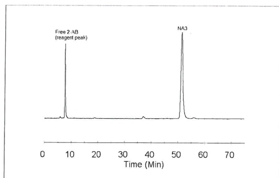
Figure 1 - HPLC of 2-AB labeled NA3
