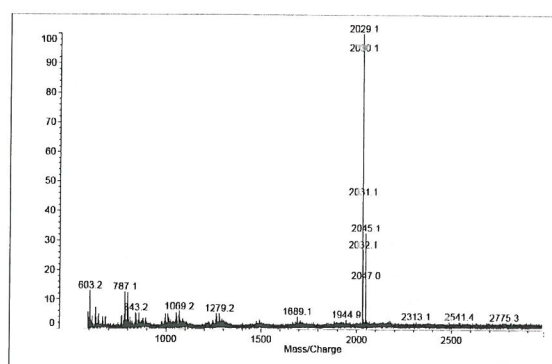
Figure 2 - MALDI-TOF of NA3 [M + Na] +
