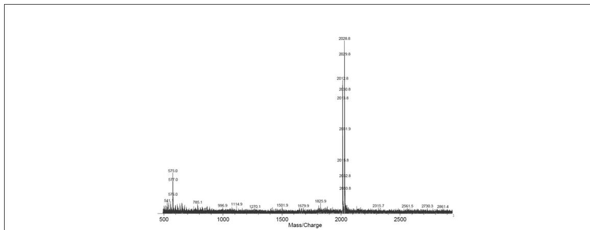
Figure 2 - Mass Spectrum of NA2FB [M + Na] +
