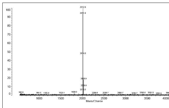
Figure 2 - MALDI-TOF mass spec of NA2FB [M + Na] +
