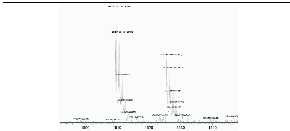
Figure 2 - Mass Spectrum of NA2F [M+Na] +
