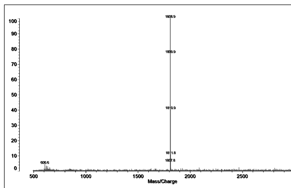
Figure 2 - MALDI-TOF mass spec of NA2F [M + Na] +
