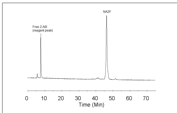
Figure 1 - HPLC results: NA2F labeled according to the Signal™ 2-AB Labeling Kit (GKK-404) and analyzed on a GlycoSep™ N column (GKI-4728) in ammonium formate/acetonitrile.
