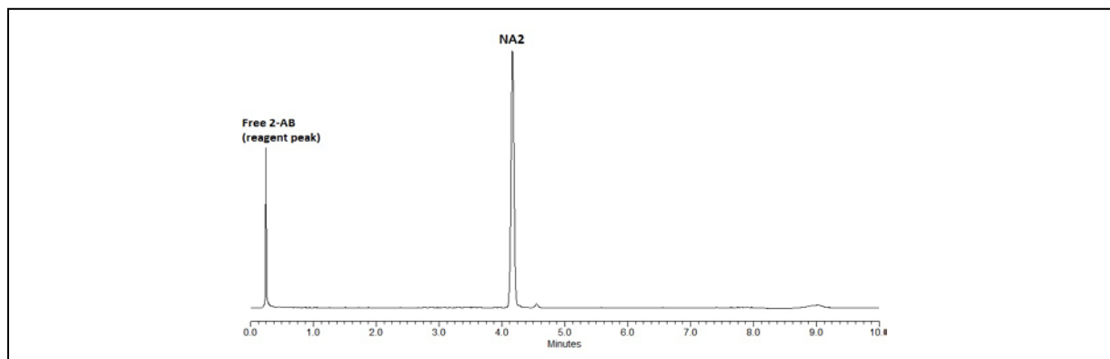
Figure 1 - UPLC® Results: 3 - 6 pmol (1 µl, aqueous) of the 2-AB-labeled glycan was injected on a Waters ACQUITY UPLC® H Class System utilizing a 10-minute method under the conditions below:
