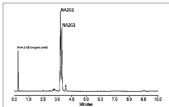
Figure 3 - NA2G1 labeled according to the Signal™ 2-AB Labeling Kit (GKK-404) and analyzed on a Waters ACQUITY® UPLC® BEH Glycan column (1.7 μm, 2.1 x 100 mm) in ammonium formate/acetonitrile.
