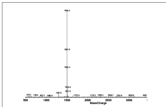
Figure 2 - MALDI-TOF mass spec of NA2G1 [M + Na] +
