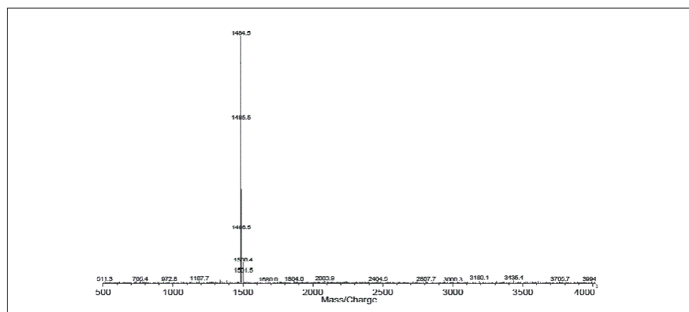
Figure 2 - Mass Spectrum of NGA2F [M + Na] +
