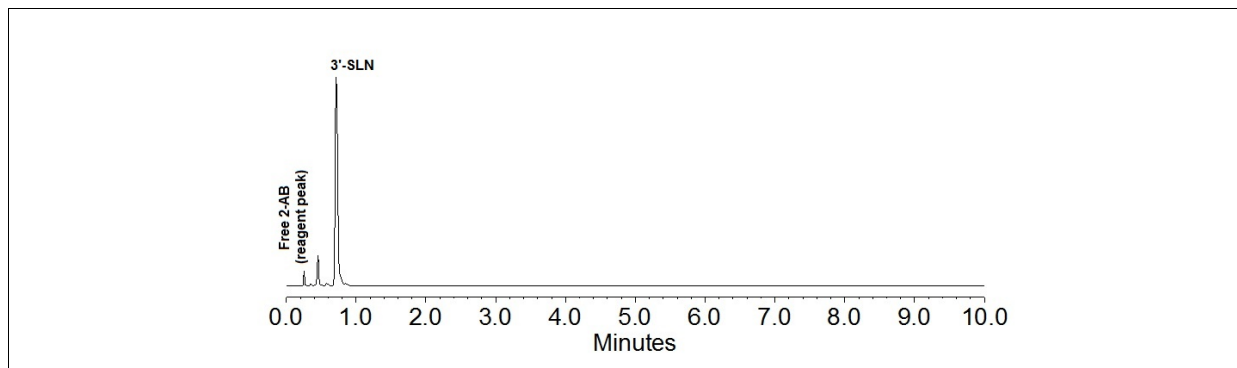
Figure 1 - UPLC® Results: 11 - 12 pmol (1 µl, aqueous) of the 2-AB-labeled glycan was injected on a Waters ACQUITY UPLC® H Class System utilizing a 10-minute method under the conditions below:
