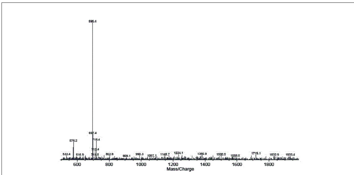
Figure 2 - Mass Spectrum of 3'-SLN
