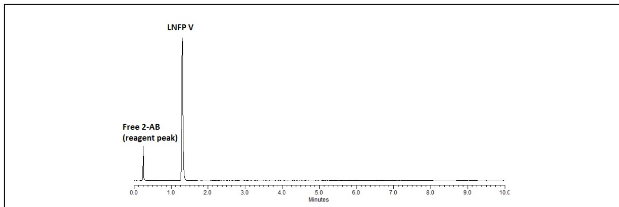
Figure 1 - UPLC® Results: 7 - 11 pmol (1 µl, aqueous) of the 2-AB-labeled 4 glycan was injected on a Waters ACQUITY UPLC® H Class System utilizing a 10-minute method under the conditions below:
