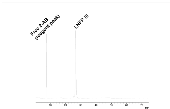
Figure 1 - HPLC results: LNFP III labeled according to the Signal™ 2-AB Labeling Kit (GKK-404) and analyzed on a GlycoSep™ N column (GKI-4728) in ammonium formate/acetonitrile.
