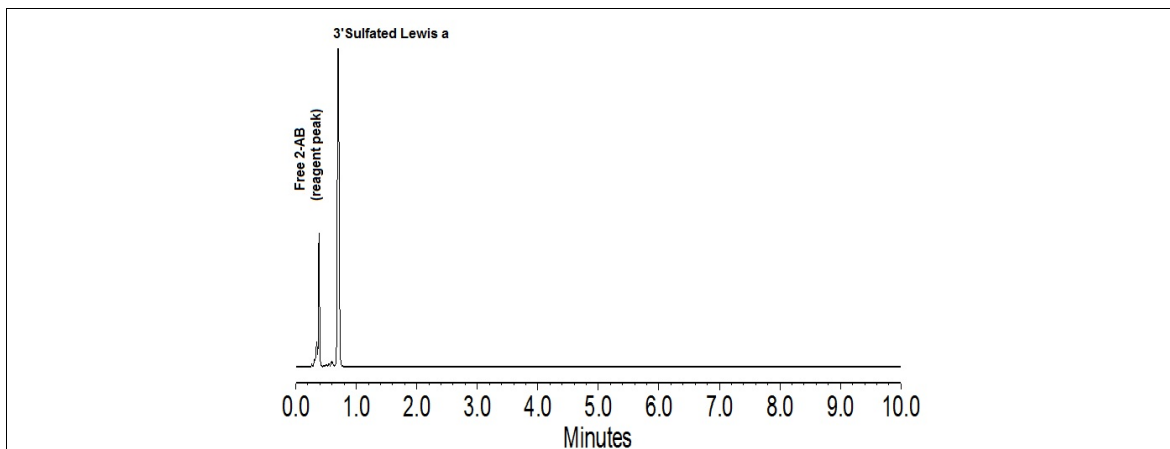
Figure 1 - UPLC® Results: 3 - 6 pmol (1 µl, aqueous) of the 2-AB-labeled glycan was injected on a Waters ACQUITY UPLC® H Class System utilizing a 10-minute method under the conditions below:
