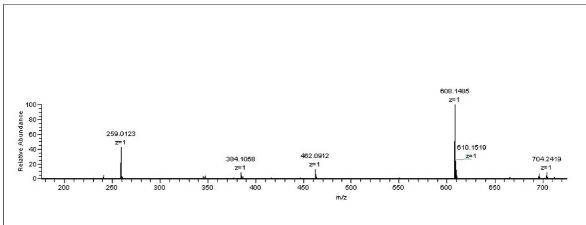
Figure 2 - Mass Spectrum of 3'-SO 3 H-Le a
