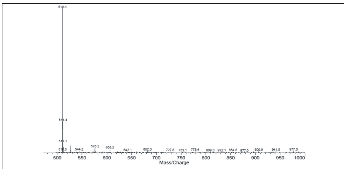
Figure 2 - Mass Spectrum of Blood Group B
