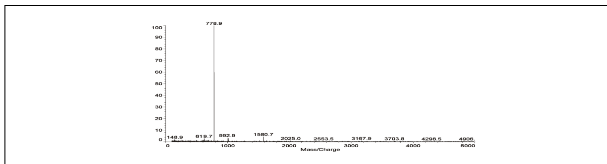
Figure 2 - Mass Spectrum of 3'-S, 3-FL
