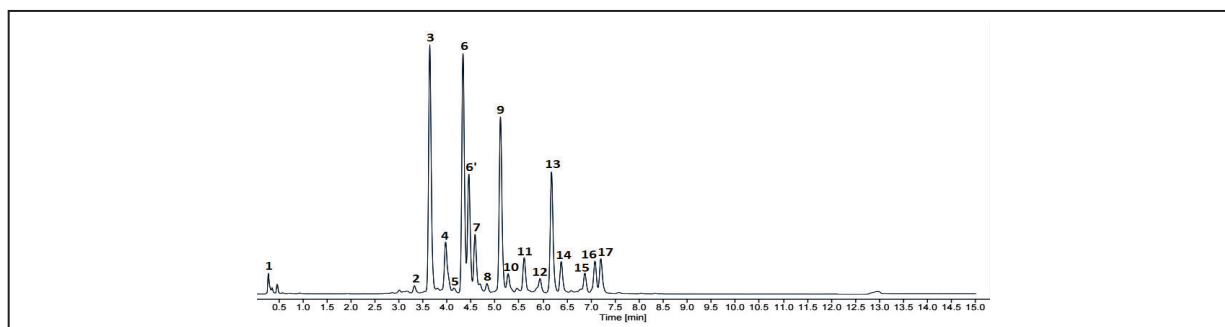
Figure 1 - UHPLC Results: 1 \mu L, aqueous of the InstantPC-labeled glycan was injected on a UHPLC System (Agilent 1290 Infinity II) utilizing a 15-minute method under the conditions below (see Table 1 for peak ID; the number of peaks observed depends on the running conditions employed):
